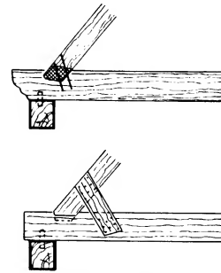
③ Repair of a coupled roof using plastic joints or wooden joint splicing
